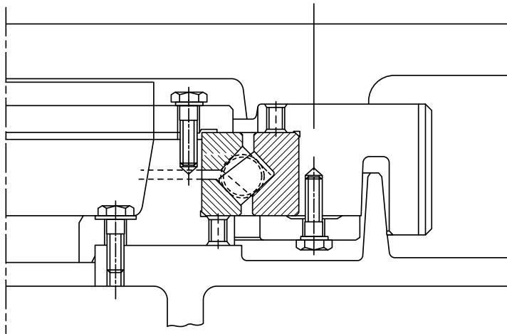
Fig. 123. Typical mounting arrangement of a TXRDO bearing.
