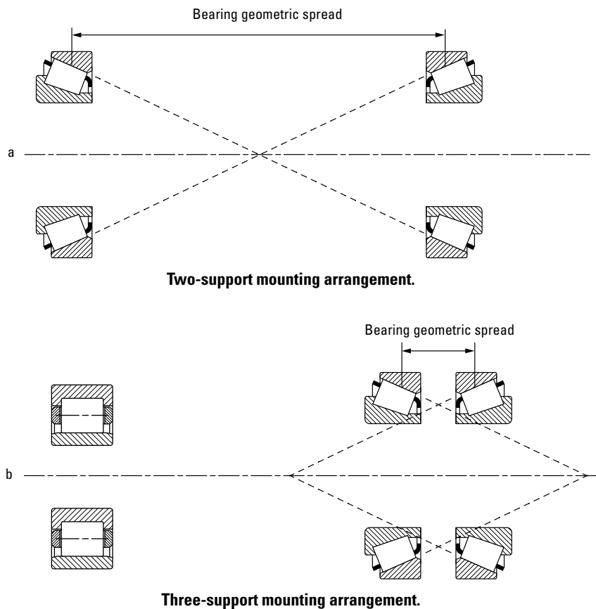
Fig. 137. Mounting arrangements.
