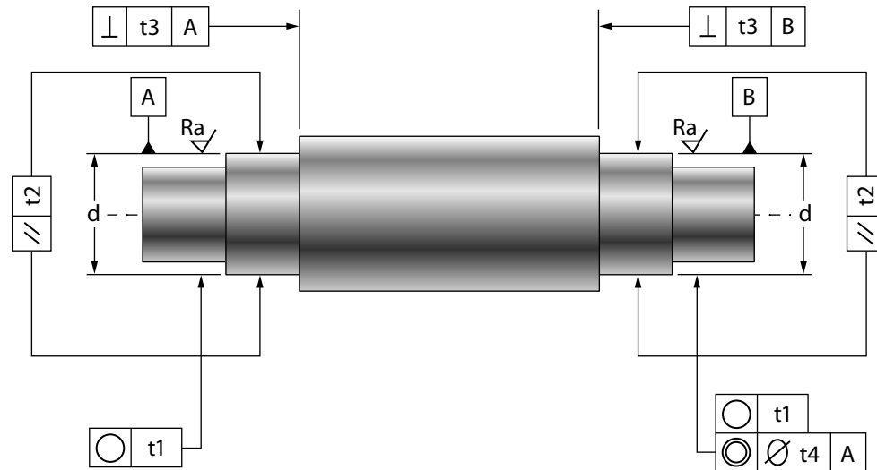
Shaft tolerances
