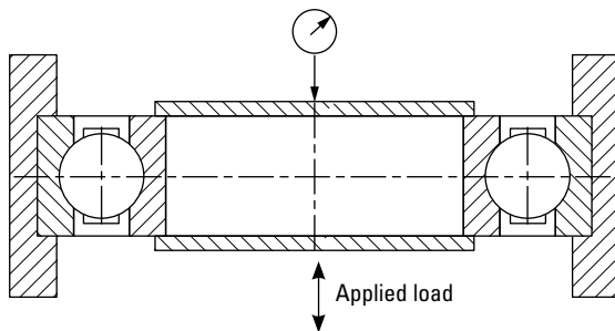
Fig. 112. Example of endplay.
